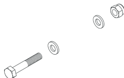
8x M6 x 35 hex head bolt 16x M6 washer 24x M6 nyloc nut (TT1-SK only)
